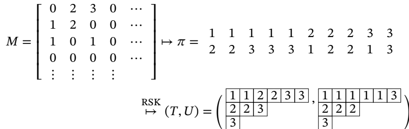
Figure 7.13. The Robinson–Schensted–Knuth map
