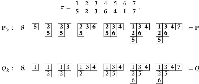
Figure 7.12. The Robinson–Schensted map
