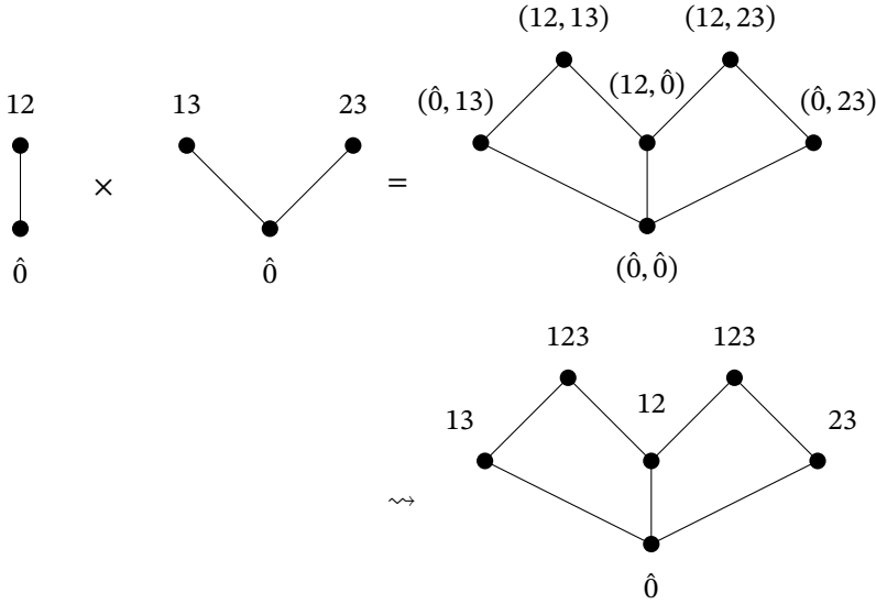
Figure 5.11. A product of claws with partition labels
