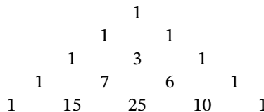
Figure 1.3. Rows 1 through 5 of Stirling's second triangle
